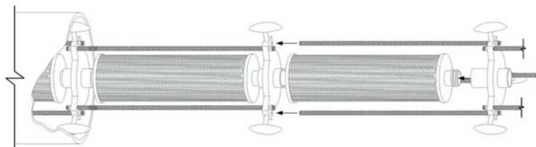
TYPICAL FILTER SUPPORT SYSTEM
