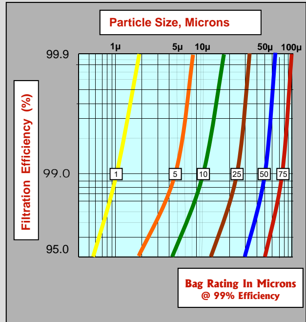
EFFICIENCY CURVES
